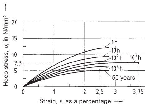
Figure 2: Stress-strain diagram for PE 80 at 20 °C
