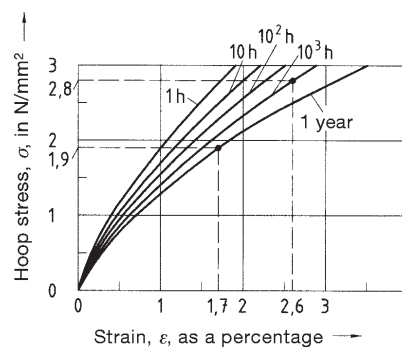
Figure 5: Stress-strain diagram for PE 100 at 80 °C
