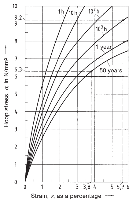
Figure 4: Stress-strain diagram for PE 100 at 20 °C
