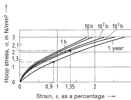
Figure 3: Stress-strain diagram for PE 80 at 80 °C
