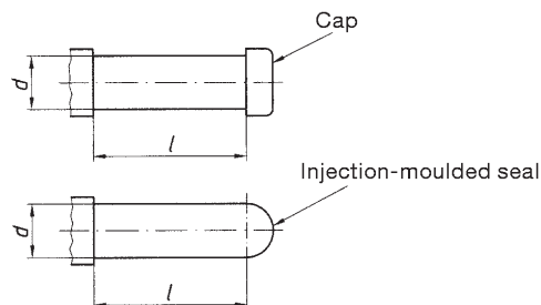
Figure 1: Form of test pieces
